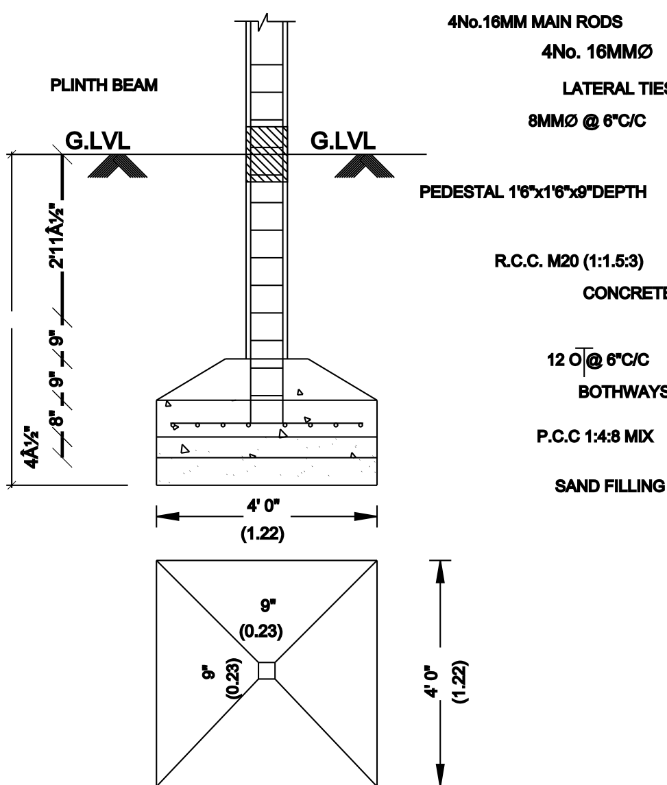
FOUNDATION DETAIL (SCALE: 1/8)
