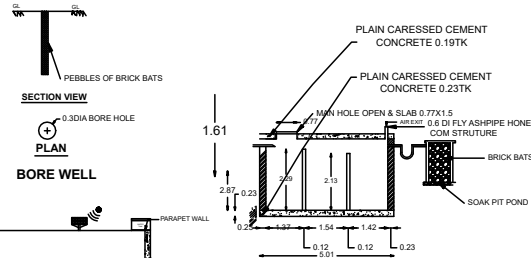
SECTION XX
