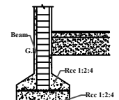
SECTION Z-Z
