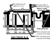
DETAIL OF SEPTIC TANK
