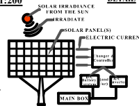
SOLAR PANEL
