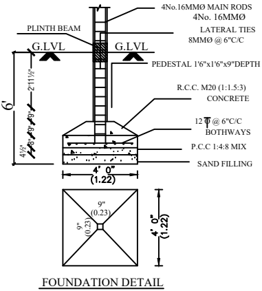
FOUNDATION DETAIL
