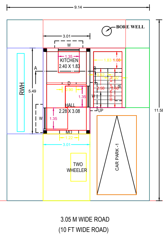
SITE CUM PRO.GROUND FLOOR PLAN
