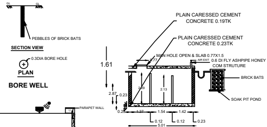
SECTION XX
