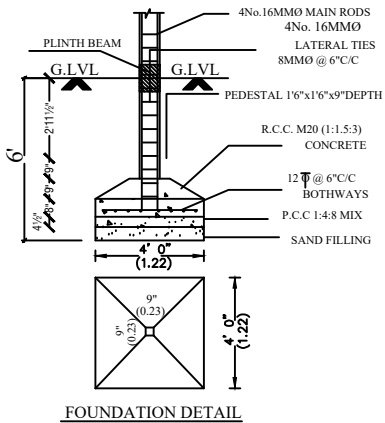
FOUNDATION DETAIL
