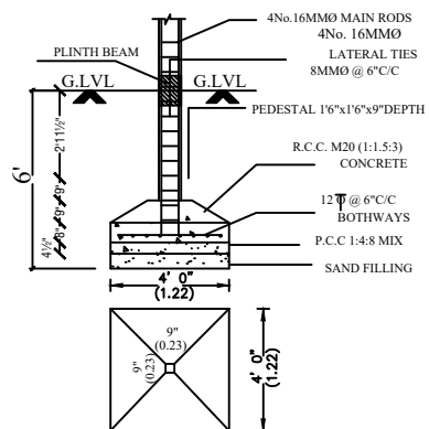
FOUNDATION DETAIL
