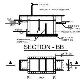
(23) (244) (23) PLAN OF SEPTIC TANK
