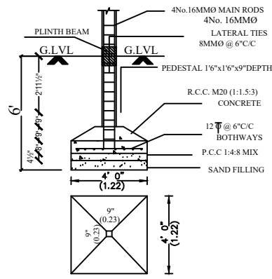
FOUNDATION DETAIL
