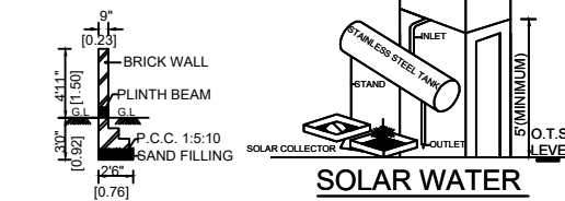
SECTION - CC
