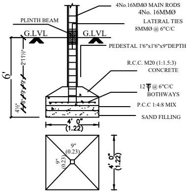
FOUNDATION DETAIL
