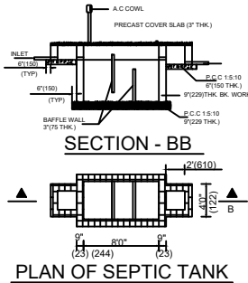
SECTION - BB PLAN OF SEPTIC TANK
