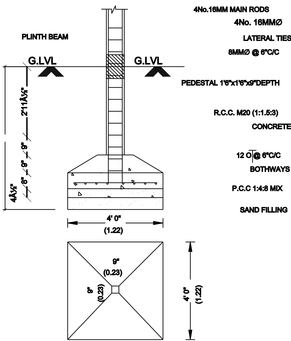
FOUNDATION DETAIL
