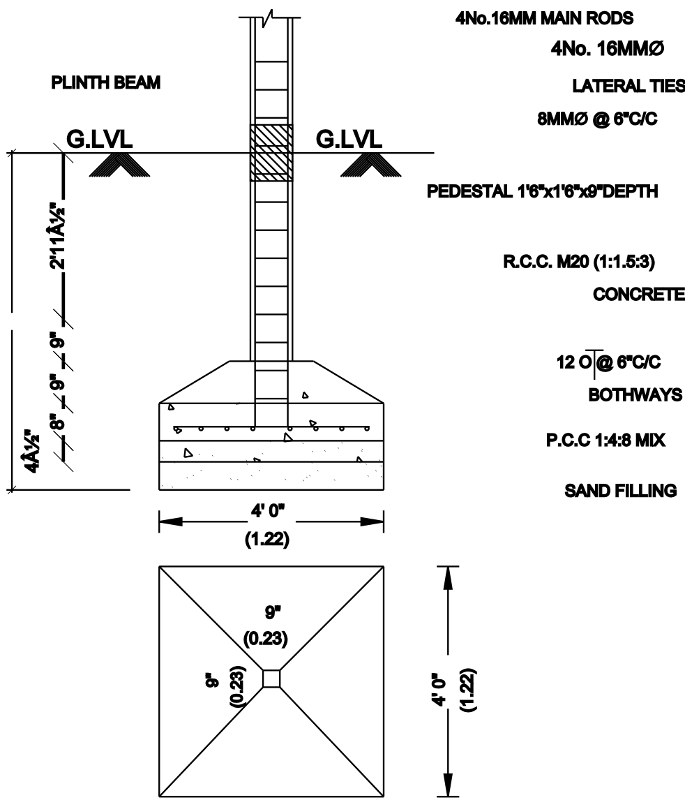
FOUNDATION DETAIL
