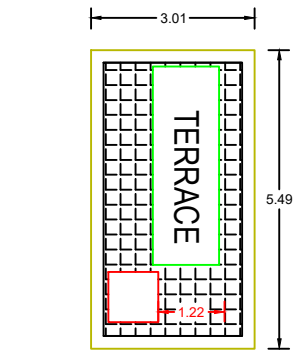
PRO. TERRACE FLOOR PLAN
