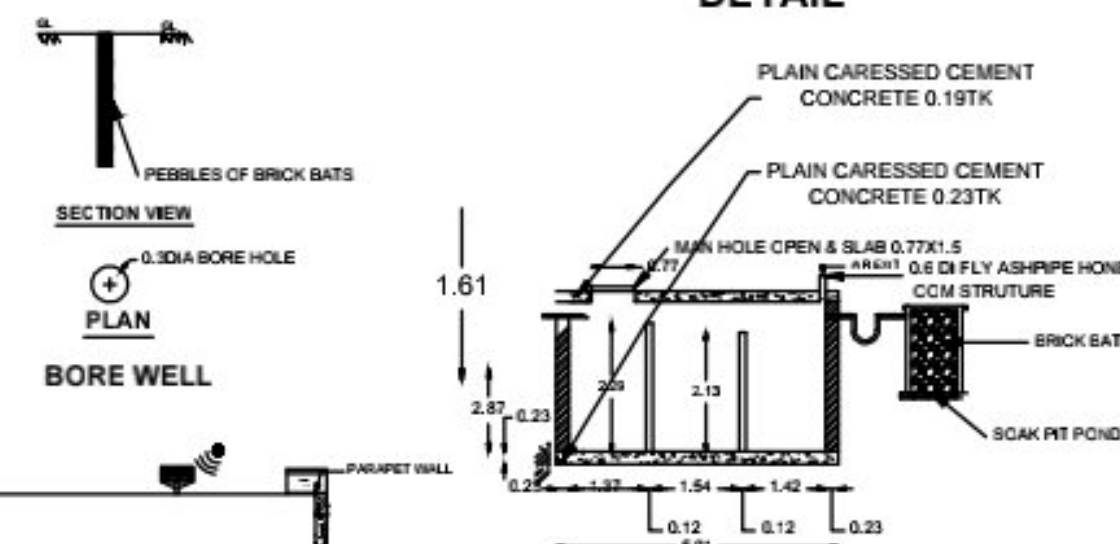
SECTION XX
