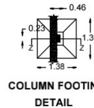
SECTION Z-Z
