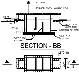
PLAN OF SEPTIC TANK
