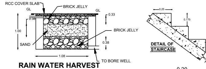
RAIN WATER HARVEST
