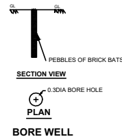
BORE WELL
