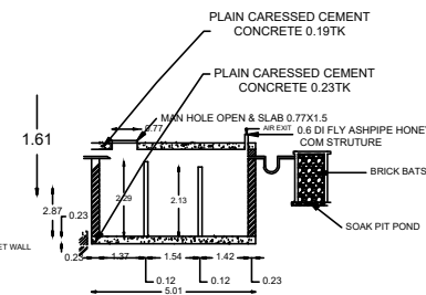
SECTION XX
