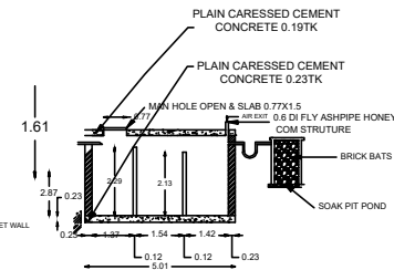
SECTION XX
