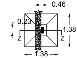
COLUMN FOOTING DETAIL
