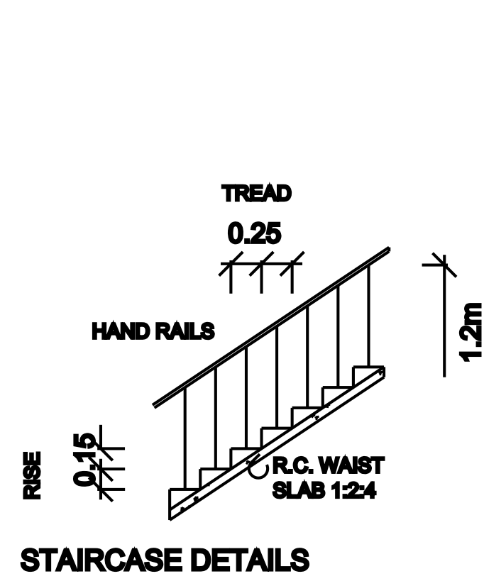
STAIRCASE DETAILS
