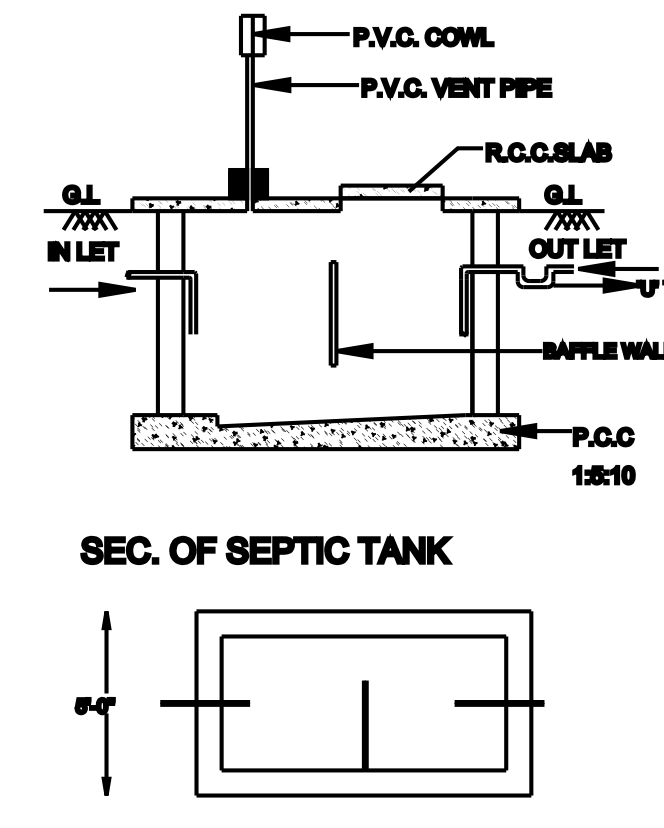
SEC. OF SEPTIC TANK
