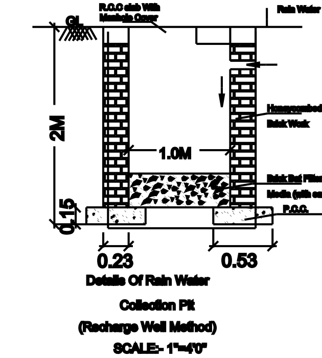
Details of Rain Water Collection (RWC) (Recharge Well Method) SCALE- 1"=4'0"
