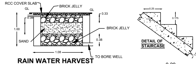
RAIN WATER HARVEST
