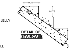
DETAIL OF STAIRCASE
