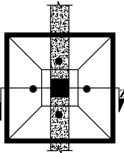
COLUMN FOOTING DETAIL
