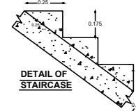
DETAIL OF STAIRCASE
