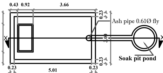
DETAIL OF SEPTIC TANK (scale -1:200)
