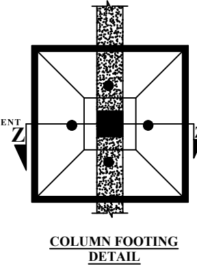
SCALE 1:200
