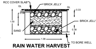
RAIN WATER HARVEST
