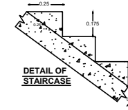
DETAIL OF STAIRCASE
