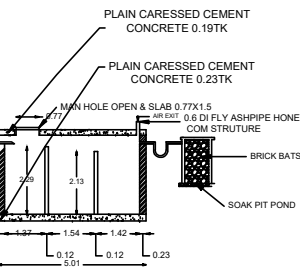
SECTION XX
