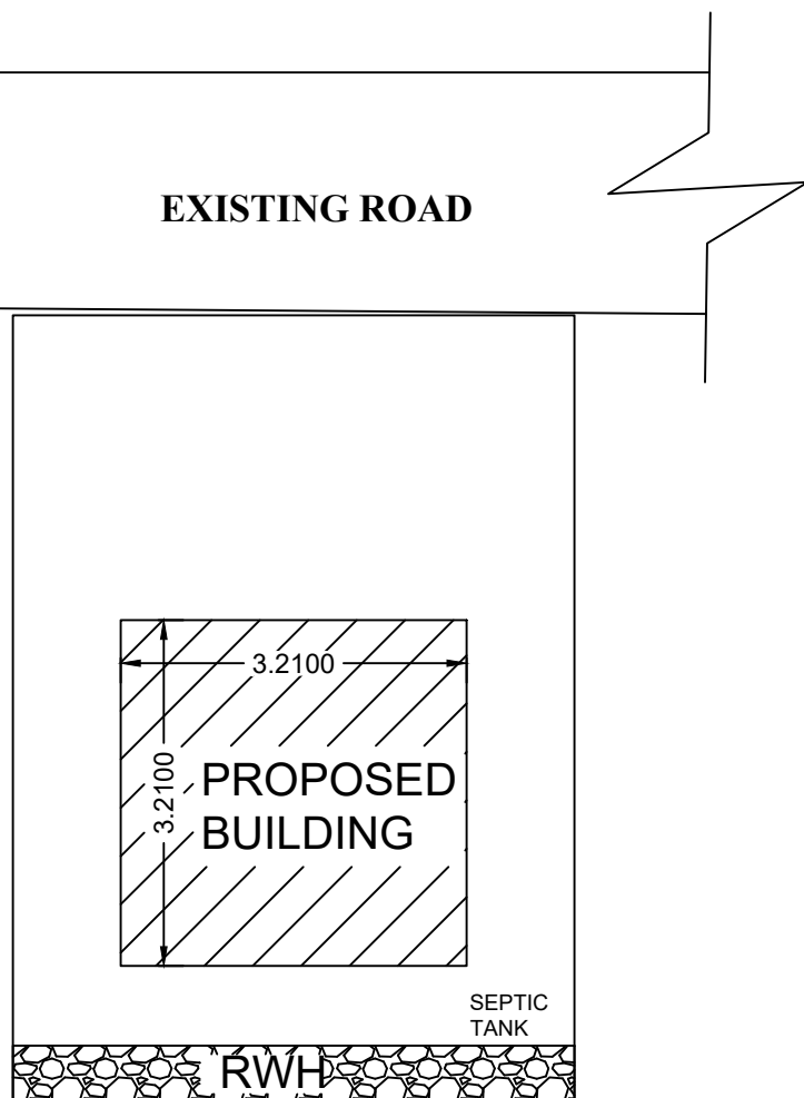
SITE PLAN
