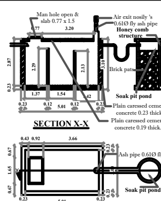
DETAIL OF SEPTIC TANK (scale -1:200)
