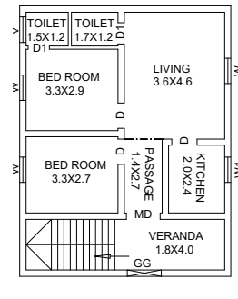
PROPOSED GROUND FLOOR
