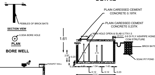
SECTION XX
