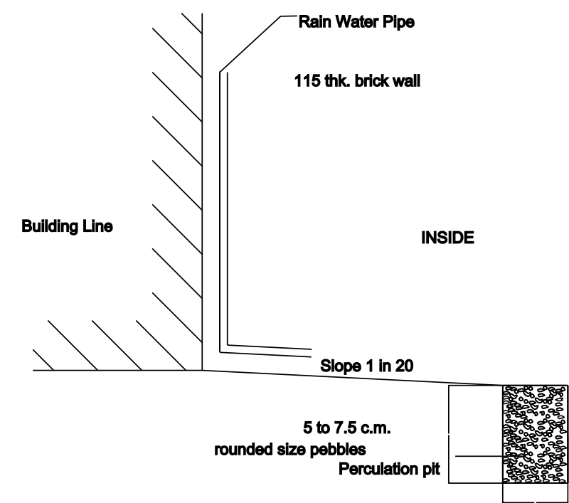
FOUNDATION DETAILS
