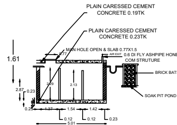
SECTION XX
