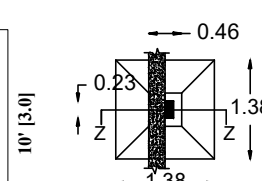
COLUMN FOOTING DETAIL
