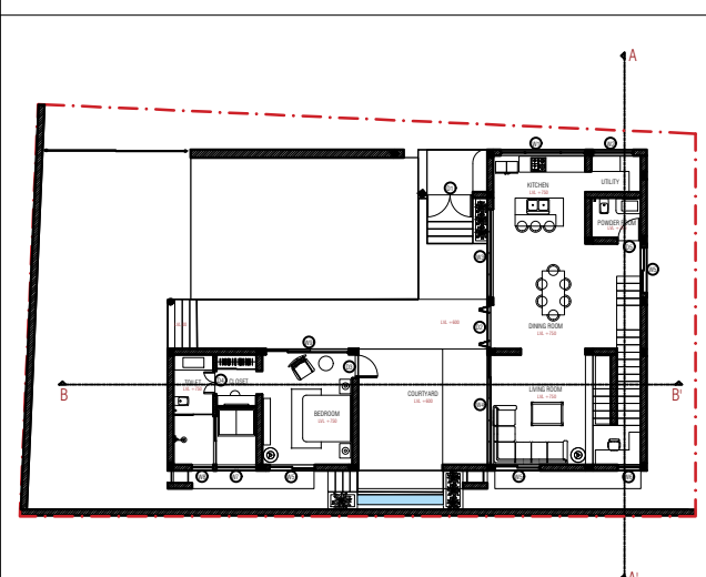
UNIT 1 GROUND FLOOR PLAN
