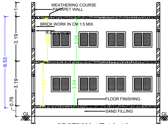
SECTION AT A1-A1
