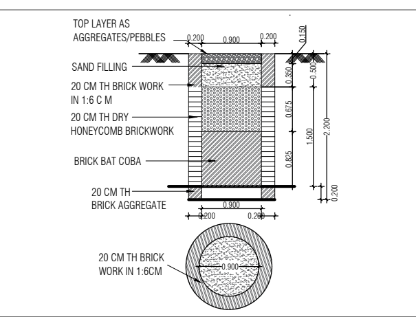
RAIN WATER HARVESTING PIT DETAIL
