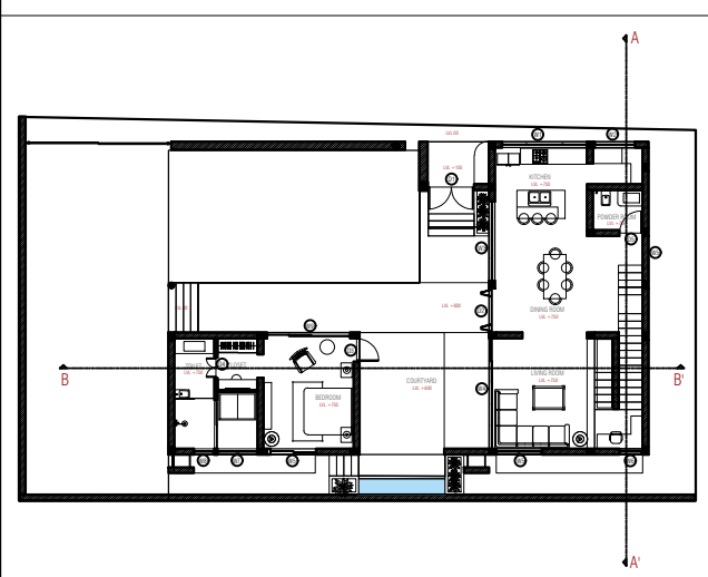
UNIT 2 GROUND FLOOR PLAN
