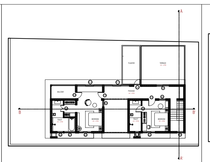
UNIT 2 FIRST FLOOR PLAN
