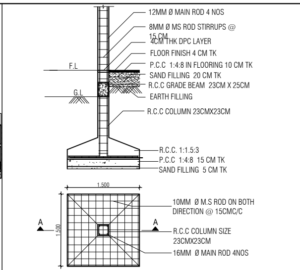
RCC FOUNDATION DETAIL
