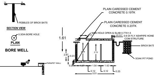
SECTION XX
