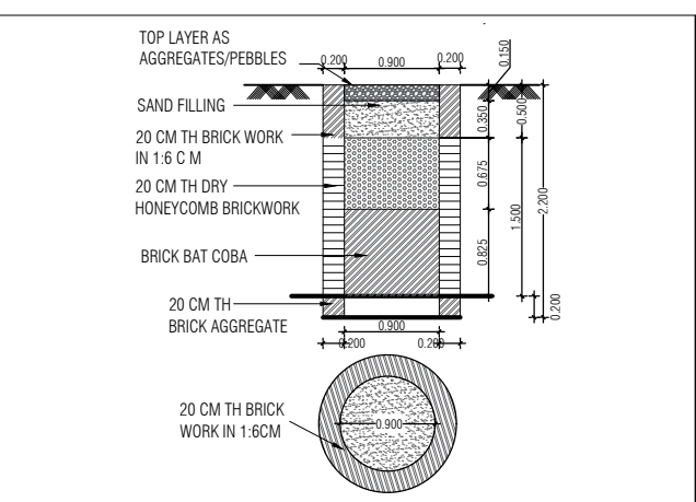
RAIN WATER HARVESTING PIT DETAIL
