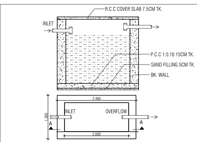
STORAGE PIT DETAIL
