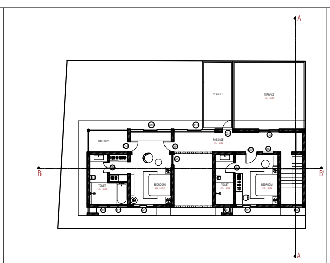
UNIT 3 FIRST FLOOR PLAN
