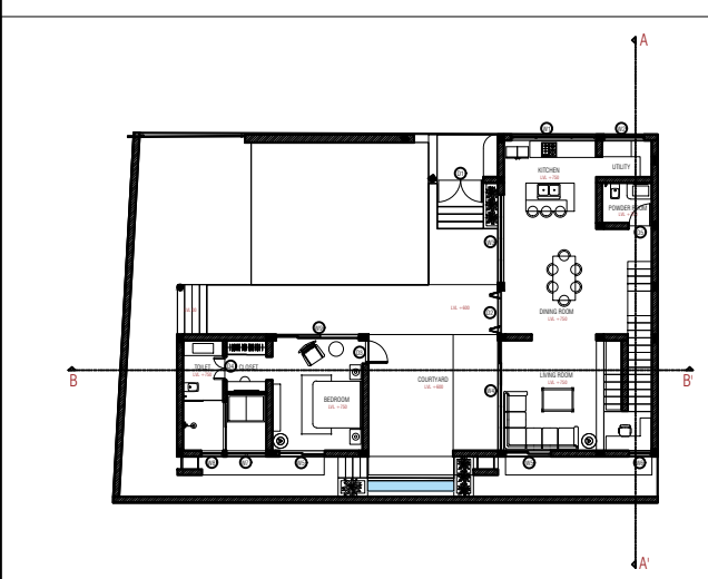
UNIT 3 GROUND FLOOR PLAN
