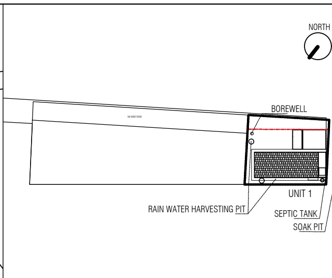
SITE PLAN
