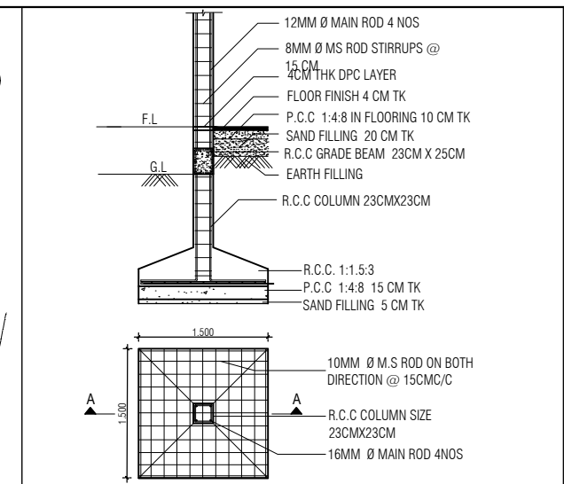
RCC FOUNDATION DETAIL
