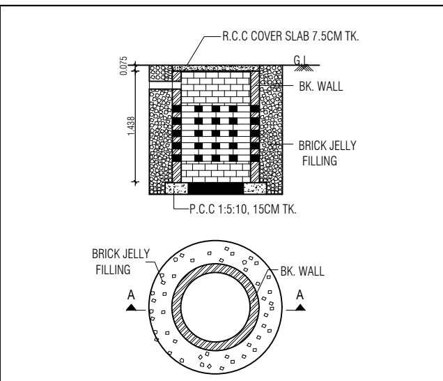
SOAK PIT DETAIL
