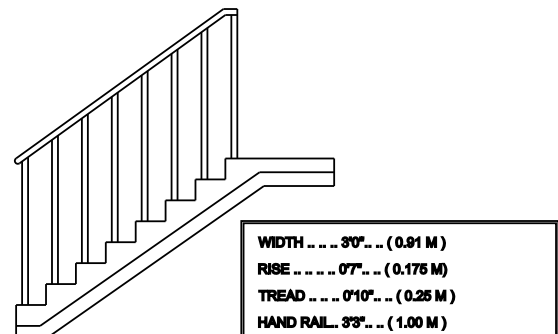
STAIR
