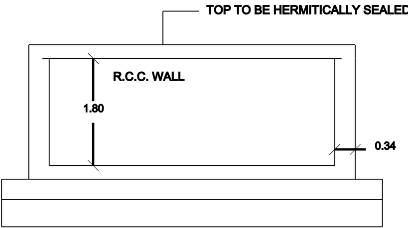
RWH SECTION (SAMPLE) RWH_CAPACITY_L=5000LTRS
