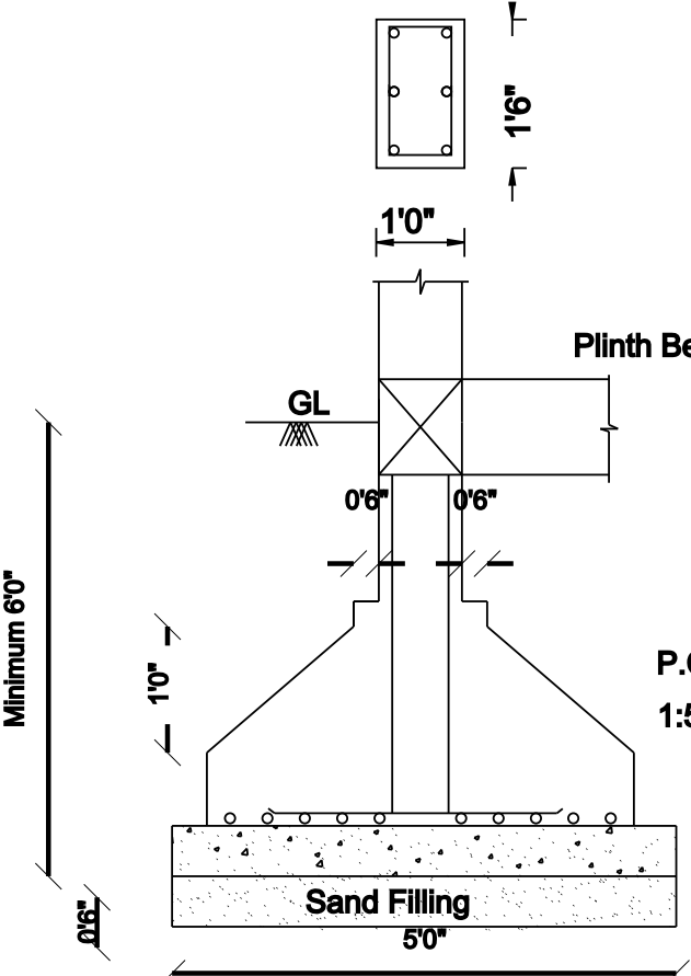
Footing Detail Column 0'9"x0'9" Not to Scale
