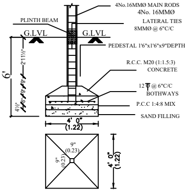
FOUNDATION DETAIL
