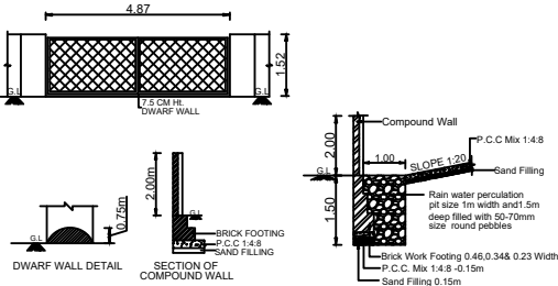
COMPOUND WALL & GATE DETAILS RAINWATER HARVESTING TRENCH
