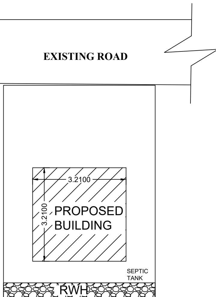
SITE PLAN
