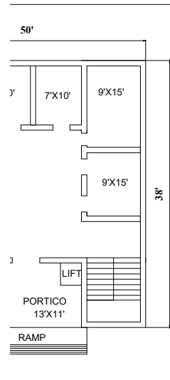
PROPOSED GROUND FLOOR
