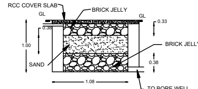
RAIN WATER HARVEST
