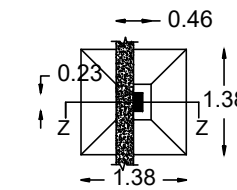
COLUMN FOOTING DETAIL
