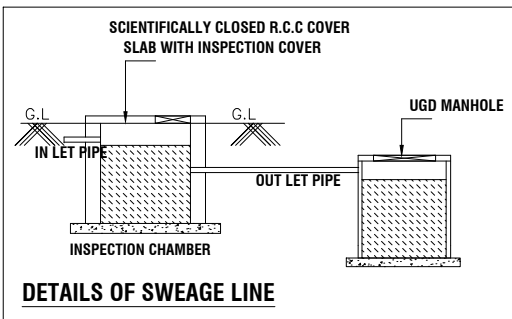
DETAILS OF SEWAGE LINE
