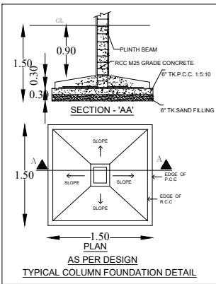
TYPICAL COLUMN FOUNDATION DETAIL
