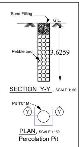
Percolation Pit
