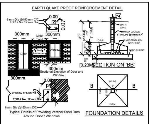
FOUNDATION DETAILS
