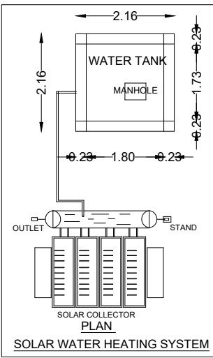
SOLAR WATER HEATING SYSTEM
