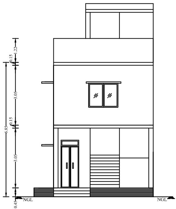
FRONT ELEVATION
