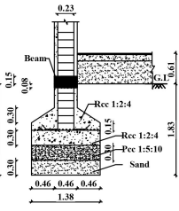
SECTION Z-Z SCALE 1:200
