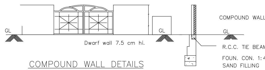
COMPOUND WALL DETAILS
