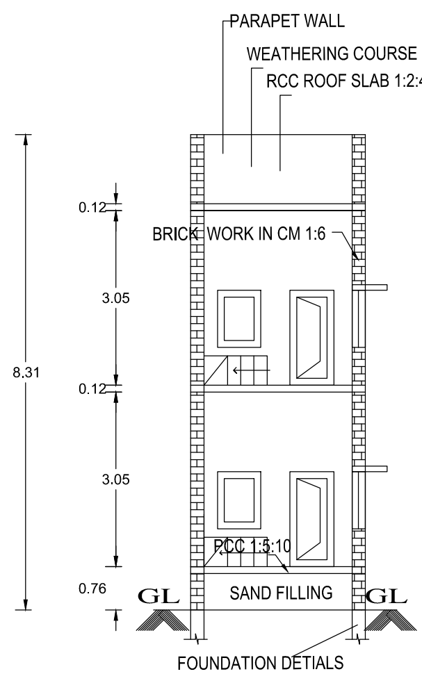
SECTION-AA'
