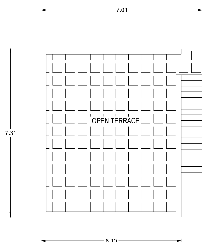
TERRACE PLAN
